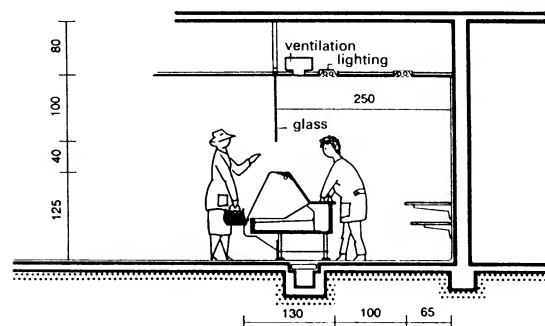
⑭ Section through counter in a self-service shop
